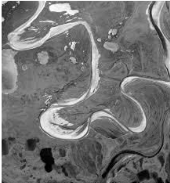
Aerial photo of a meandering stream near Barrow, AK USGS
