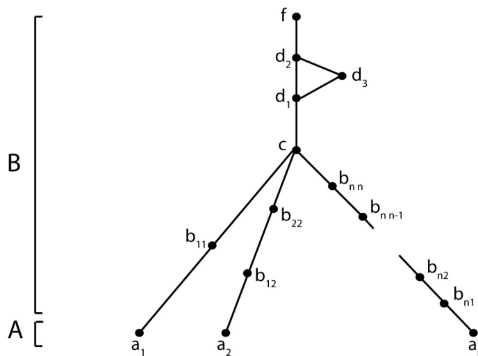
Figure 1. An n -tag T_n(a_1, \dots, a_n) .
